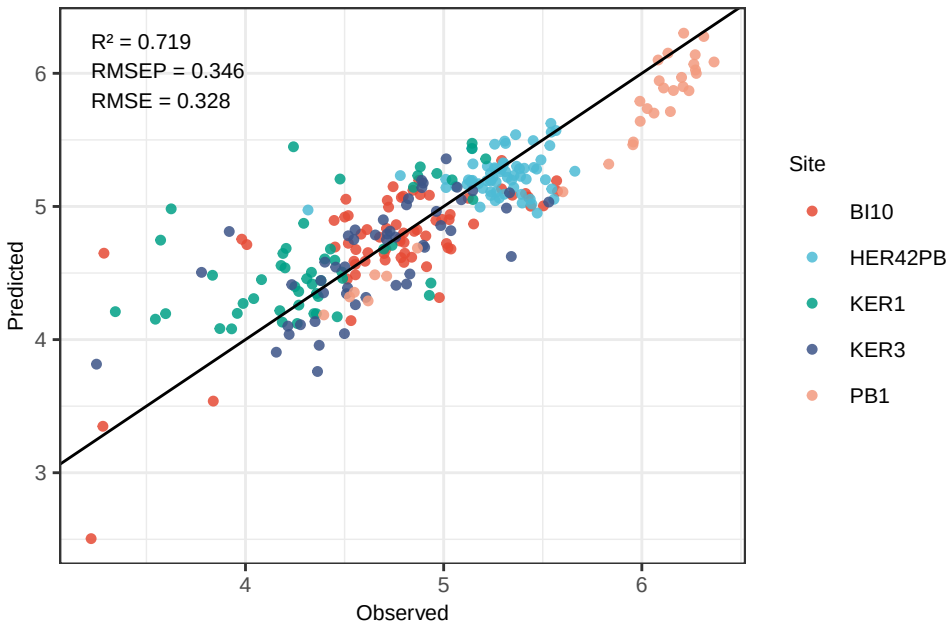
Sr Bayes – Predicted vs Observed (log-space)
